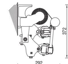
Montage korsade armar Crossed arms installation
