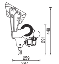
Undertaks montage Under-roof installation
